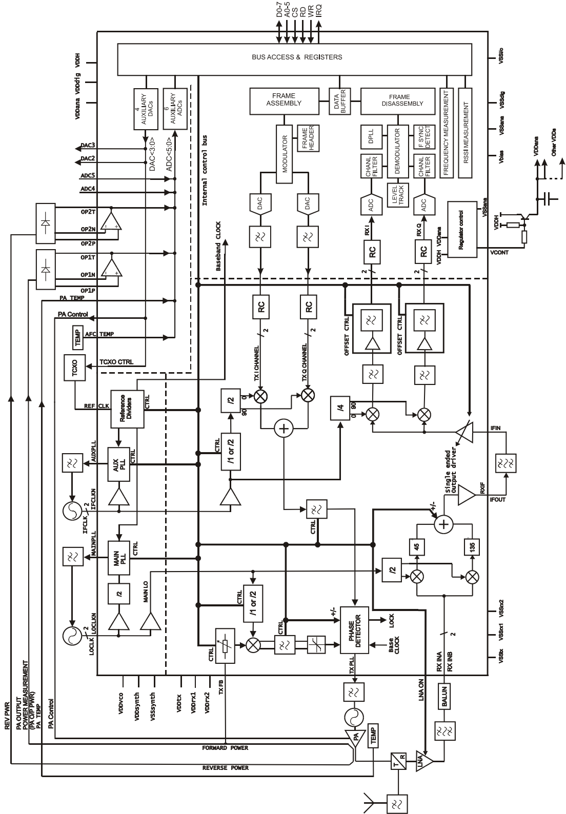
Figure 1 Block Diagram
